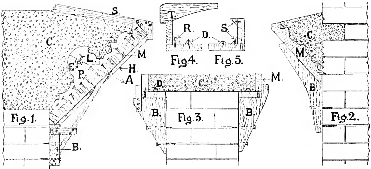
No. 203.—SECTION OF MOULDS FOR CASTING CONCRETE MOULDING "IN SITU."
